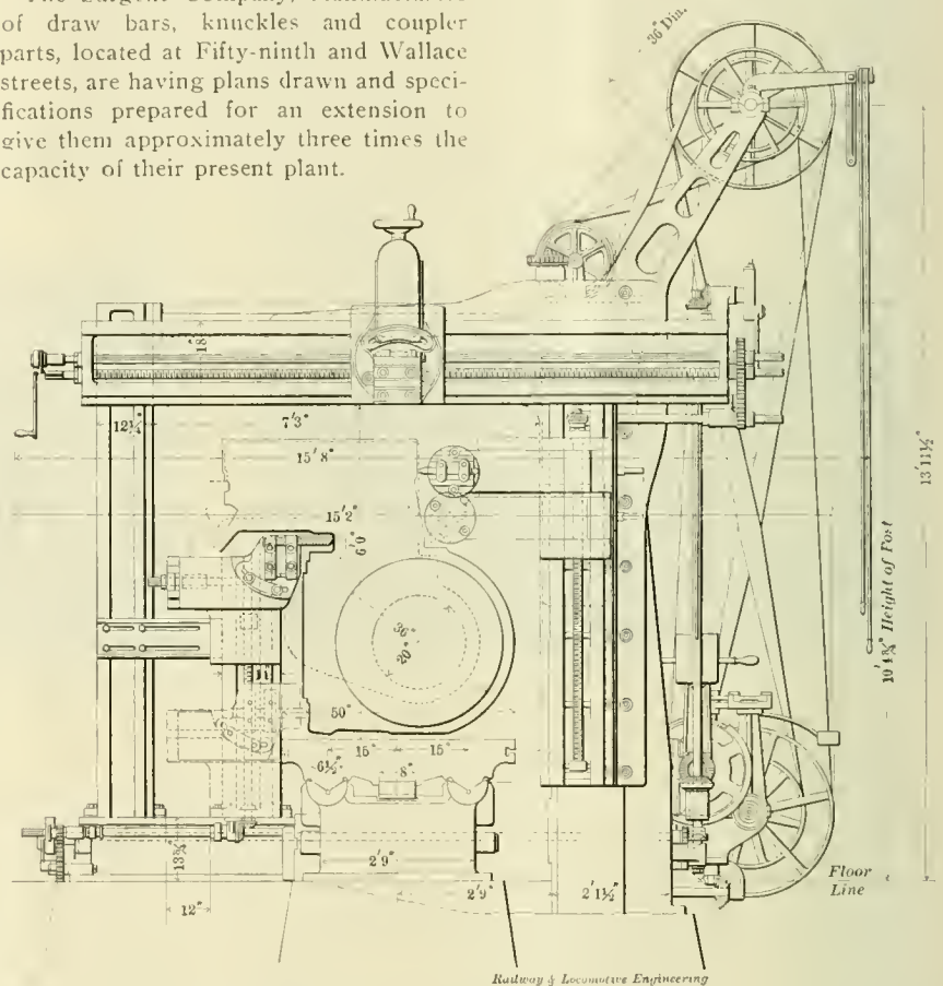
DETRICK & HARVEY CYLINDER PLANER.
